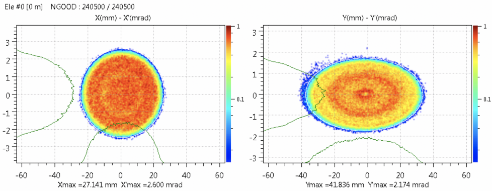
Figure 4.33: Transverse phase space of the particles used in the design of the R2S transfer line (240500 particles).
