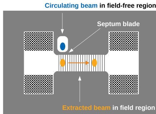
Figure 4.24: Schematic view of the Lambertson septum magnet [156]: The beam encounters no magnetic field while injection is ongoing. Once the injection is complete, the kicker magnets are powered and steer the beam towards the other side of the septum blade, where the magnetic dipole field deflects the beam horizontally.
