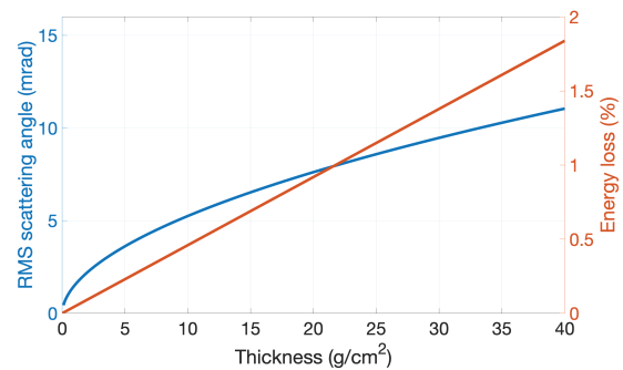
Figure 4.18: RMS scattering angle and energy loss for 2.5 GeV protons interacting with different thicknesses of tantalum.
