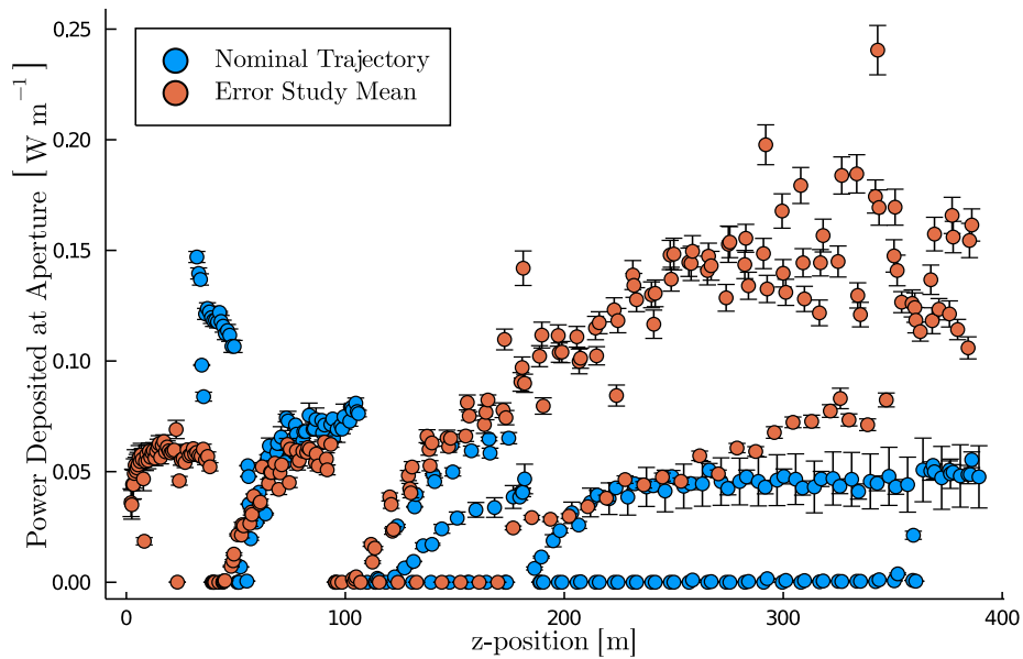
Figure 3.24: Power deposition of H^0 into beam-pipe and machine element walls for a 62.5 mA H^- beam accelerating to 2.5 GeV for the ESS \nu SB linac. Only IBSt is accounted for.
