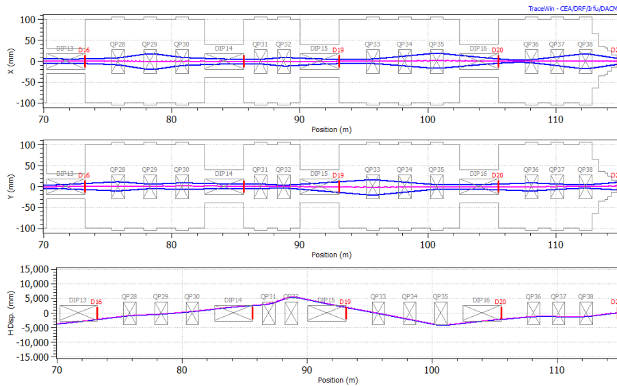
Figure 4.47: RMS transverse beam envelopes and dispersion along the T3 branch of the BSY when two quadrupoles, Q34 and Q37, are not functioning (failure scenario).
