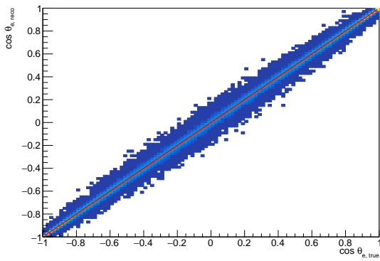
(a) Electrons
