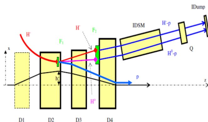
Figure 4.27: SNS injection section, shown schematically, where F1 is the stripper foil; F2 is a second, thick stripper foil to fully strip H^- and H^0 to protons; IDSM is the Injection Dump Septum Magnet; and Q is a defocusing quadrupole. From: [172].
