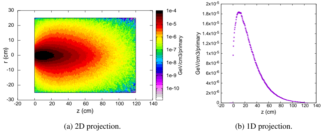
Figure 4.28: Distribution of energy loss in the copper beam dump.
