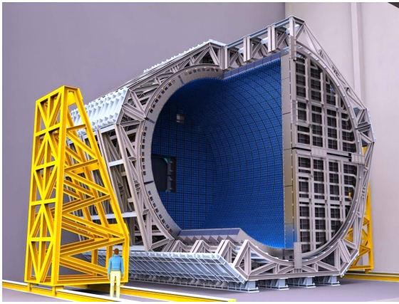
(c) An illustration of the detector structure in a mounting phase. Note the window with the interface to the SFGD.
