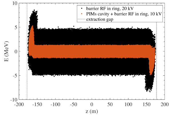
Figure 4.15: The longitudinal particle distribution at the end of injection. If the incoming energy spread is large, i.e. the case of having no cavities in the transfer line (see Fig. 4.14), it takes a barrier RF cavity with a voltage of 20 kV to preserve the extraction gap, the border of which is marked with the vertical dotted lines. With a reduced incoming spread, 5-10 kV are enough.
