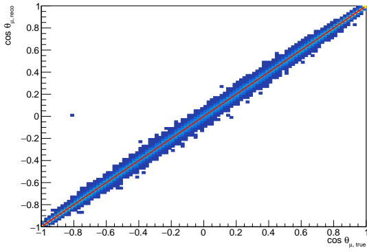
(c) Muons
