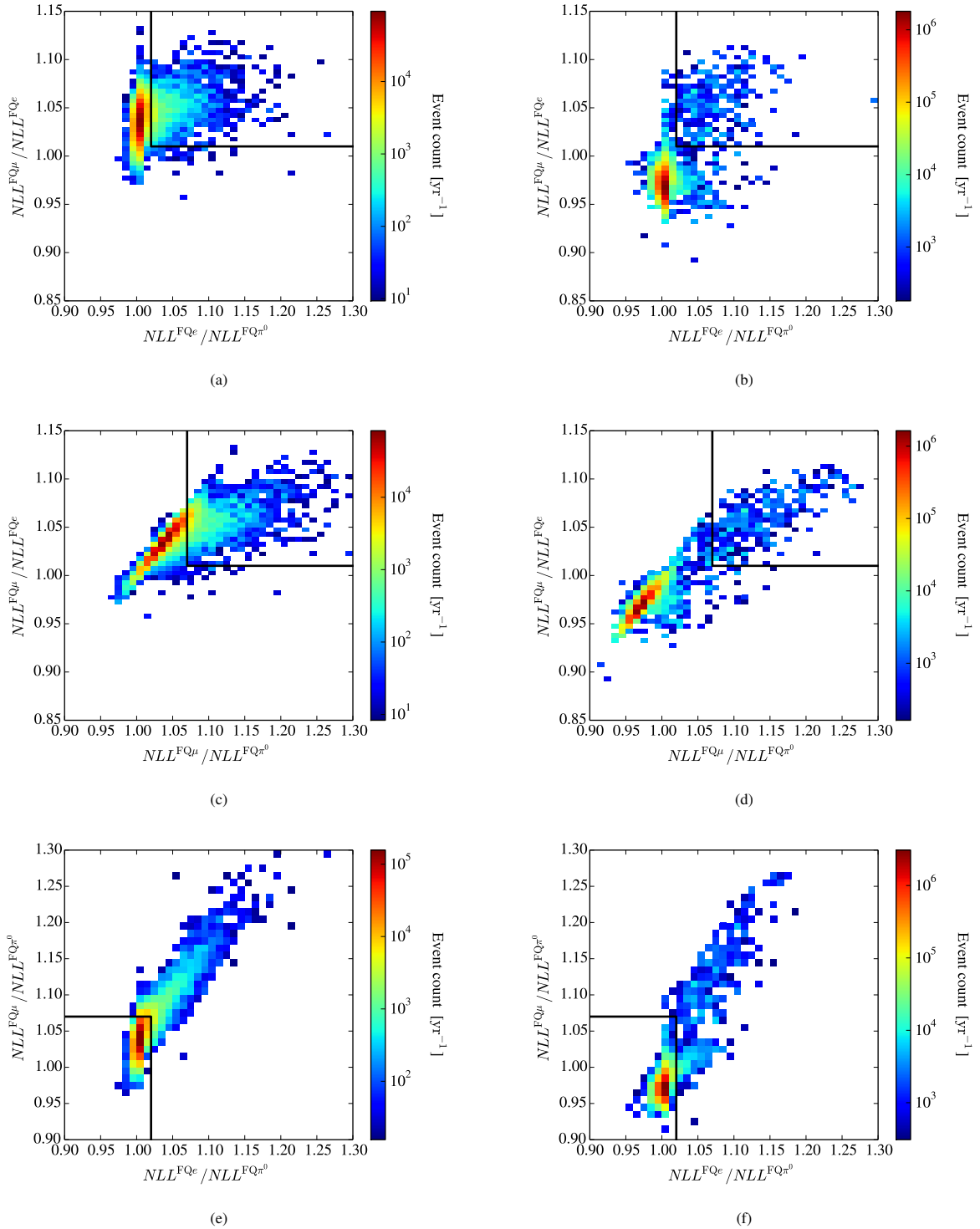
Figure 6.15: Event distributions for electron (a, c, e) and muon (b, d, f) events over the NLL^{FQ\mu} / NLL^{FQe} and NLL^{FQe} / NLL^{FQ\pi^0} variables (a, b), along with the NLL^{FQ\mu} / NLL^{FQe} and NLL^{FQ\mu} / NLL^{FQ\pi^0} variables (c, d), and the NLL^{FQ\mu} / NLL^{FQ\pi^0} and NLL^{FQe} / NLL^{FQ\pi^0} variables (e, f). The pion-like criteria , described in Eq. (6.4), are displayed as black lines in these figures. All events falling above and to the right of these lines are rejected.
