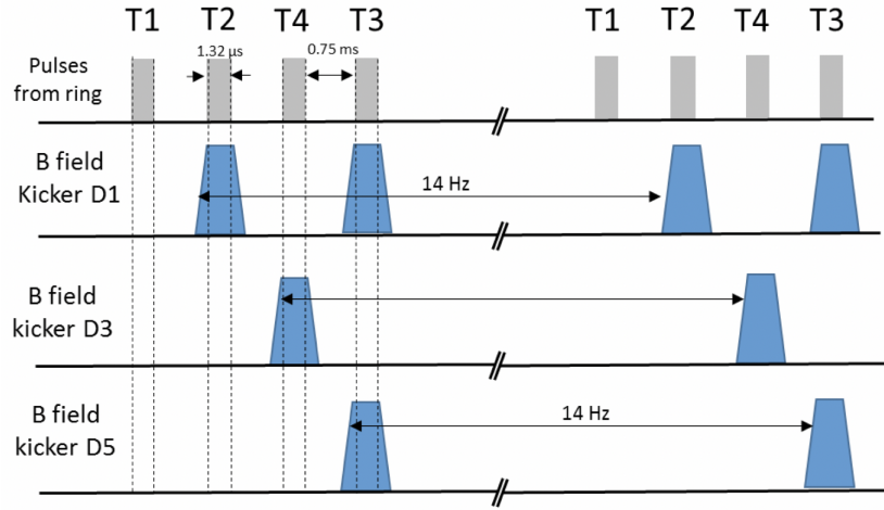
Figure 4.46: Time structure of kickers for the BSY.
