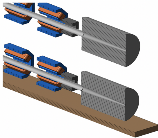
Figure 4.48: Section plane of the collimators.
