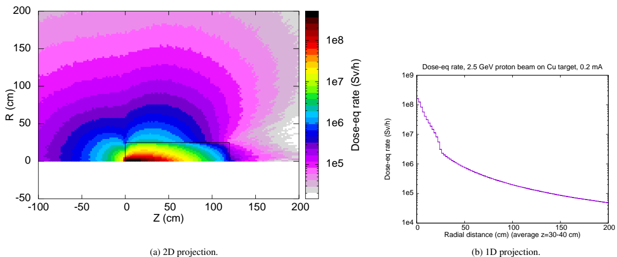
Figure 4.30: Distribution of dose-rate for source term calculations.
