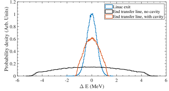
Figure 4.14: The beam energy distribution before accumulation.
