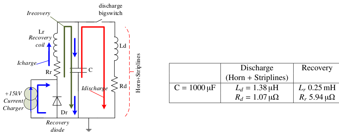
Figure 5.31: Electrical diagram for delivering 350 kA peak current during 100 μs half period (left), Electrical values of the components (right).
