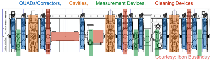
Figure 3.9: Schematic MEBT drawing with different functions indicated.
