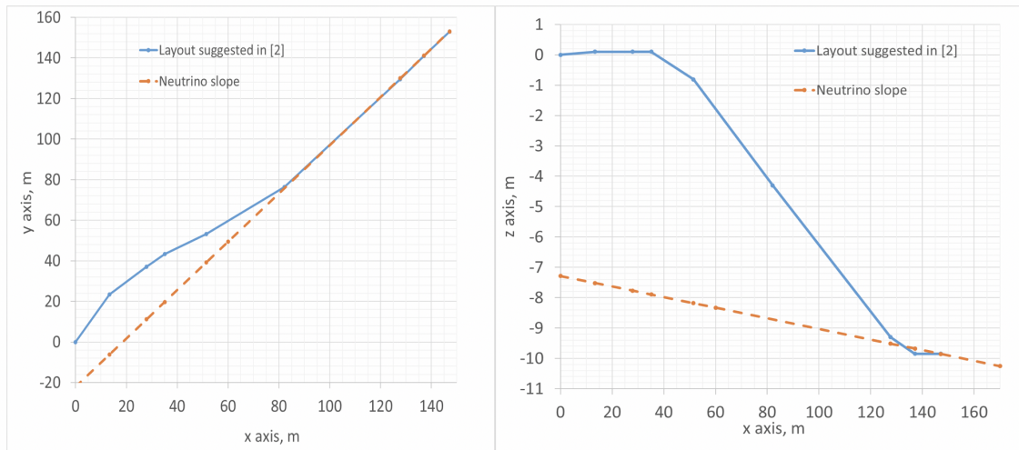
Figure 4.32: Horizontal and vertical plots of the R2S from [183] and slopes of the neutrino direction. To simplify the simulations, the extraction of the beam at the exit of the septum has the coordinates x, y, z (0; 0; 0).
