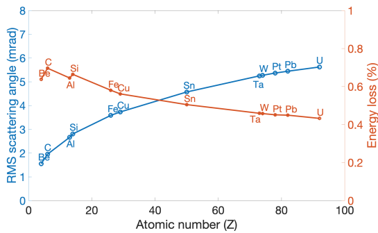
Figure 4.17: RMS scattering angle and energy loss for 2.5 GeV protons interacting with different materials, each having a thickness of 10 \text{ g}/\text{cm}^2 .
