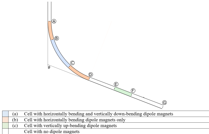
Figure 3.15: Layout of the L2R transfer line [57]. Sections are colour-coded according to the presence of horizontal and/or vertical bending
