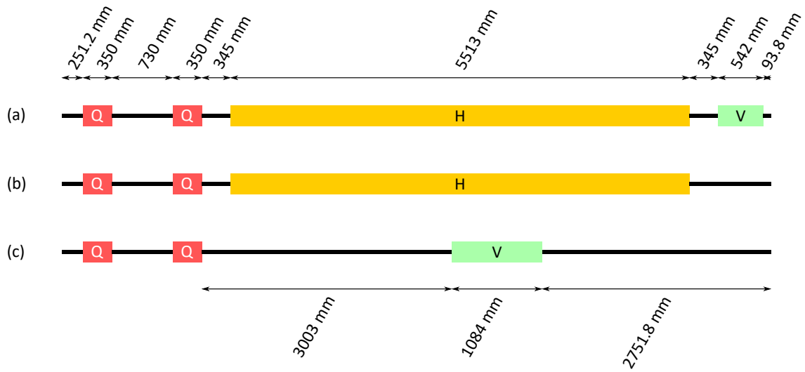
Figure 3.16: Quadrupole (Q), horizontally bending dipole (H) and vertically bending dipole (V) distributions within 8.52 m lattice cells for (a)–(c) sections listed in the legend of Fig. 3.15.
