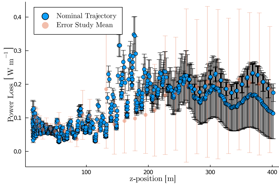
Figure 3.23: Intra-beam stripping (IBSt) power losses for a nominal trajectory and a corresponding error study for the ESS \nu SB linac ( H^- only). Static and dynamic machine errors are incorporated along with beam misalignment. Standard deviations are from the cumulative trajectories of 100 trials.
