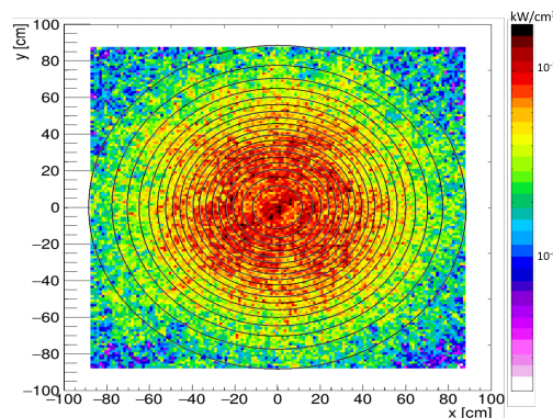
Figure 5.38: Power surface density of one horn shows a circular Gaussian distribution with \sigma \sim 36.17 cm (black circles).
