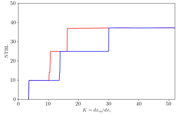
Figure 3: NBTL as a function of K for a working point with (\mu_x, \mu_y) = (87^\circ, 36^\circ) . Evolution for the nominal working point (red) and with \pm 0.5^\circ errors on both tunes (blue).
