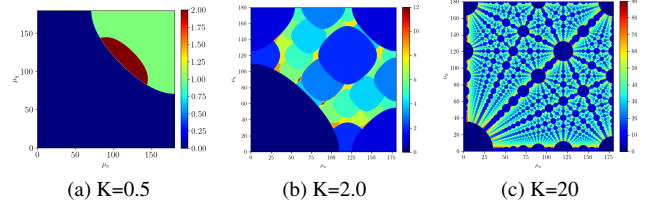
Figure 2: 3D NTBL plots in the tune diagram using Eq. (3), K from 0.5 (top-left) to 20.0 (bottom-right). Dark-blue for loss at first turn, red for the maximum NTBL values.
